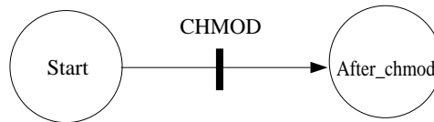
Figure 3.1: State machine
