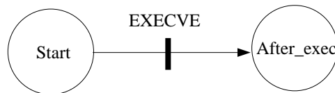
Figure 3.2: State machine
