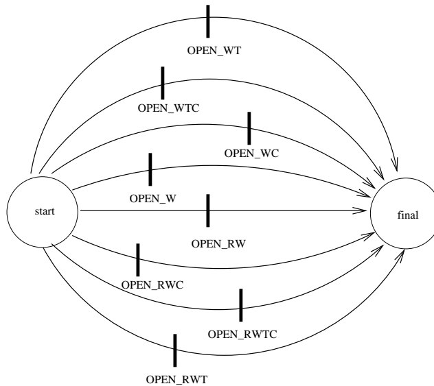
Figure 3.7: State machine for pattern to detect writing to nonowned files
