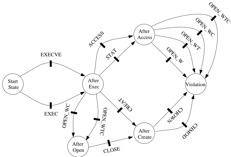
Figure 3.8: Attack state machine
